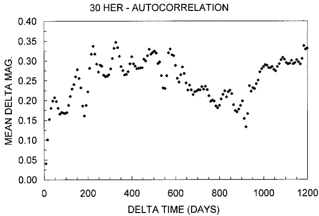
FIG. 12.—Autocorrelation diagram for 30 g Her, showing minima at multiples of 100 days, and also at 1000 days. This star shows conspicuous variations on both timescales.
