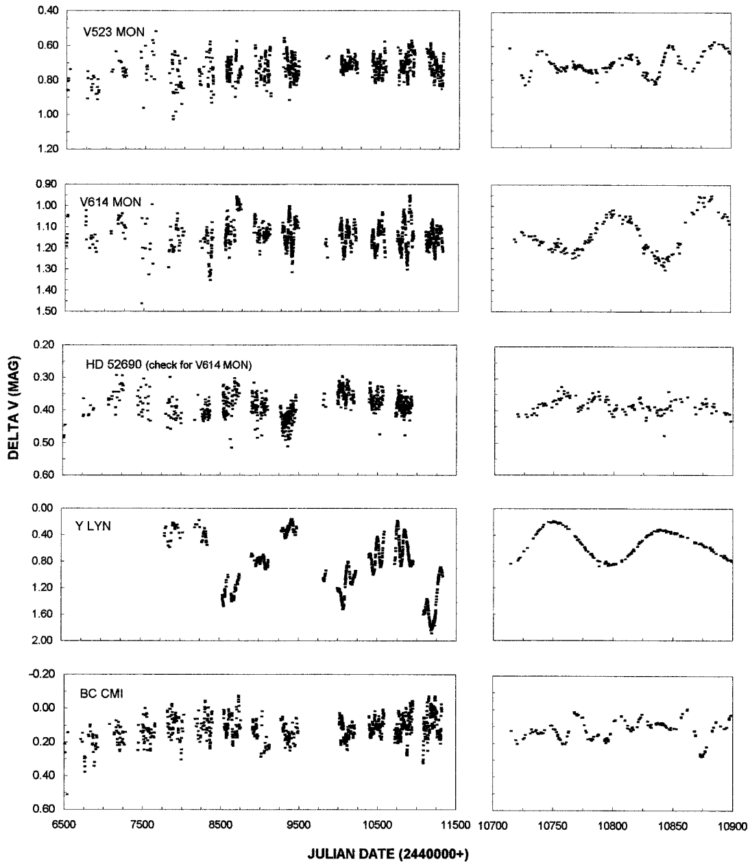
FIG. 3.—Differential V light curves of V523 Mon, V614 Mon, HD 52690 (check star for V614 Mon), Y Lyn, and BC CMI, relative to the comparison stars listed in Table 1.
