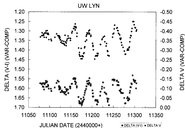
FIG. 10.—Light and color curves for UW Lyn, showing the correspondence between the V-I color curve and the V light curve, and also showing the cycle-count period of 34 days.
