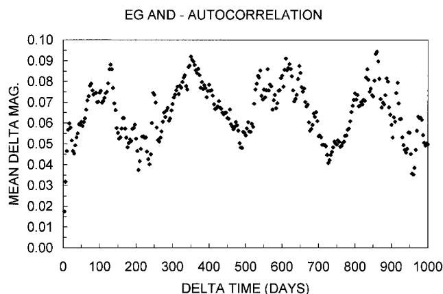
FIG. 8.—Autocorrelation diagram for EG And, showing minima at multiples of both 28 and 240 days. This star has conspicuous variations on both timescales.
