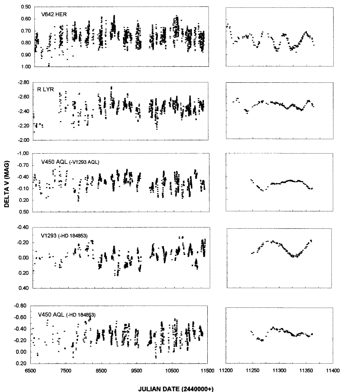
FIG. 6.—Differential V light curves of V642 Her, R Lyr, V450 Aql, and V1293 Aql, relative to the comparison stars listed in Table 1. See text for a discussion of the last two stars; in the fourth panel, V1293 is V1293 Aql, relative to the check star.
