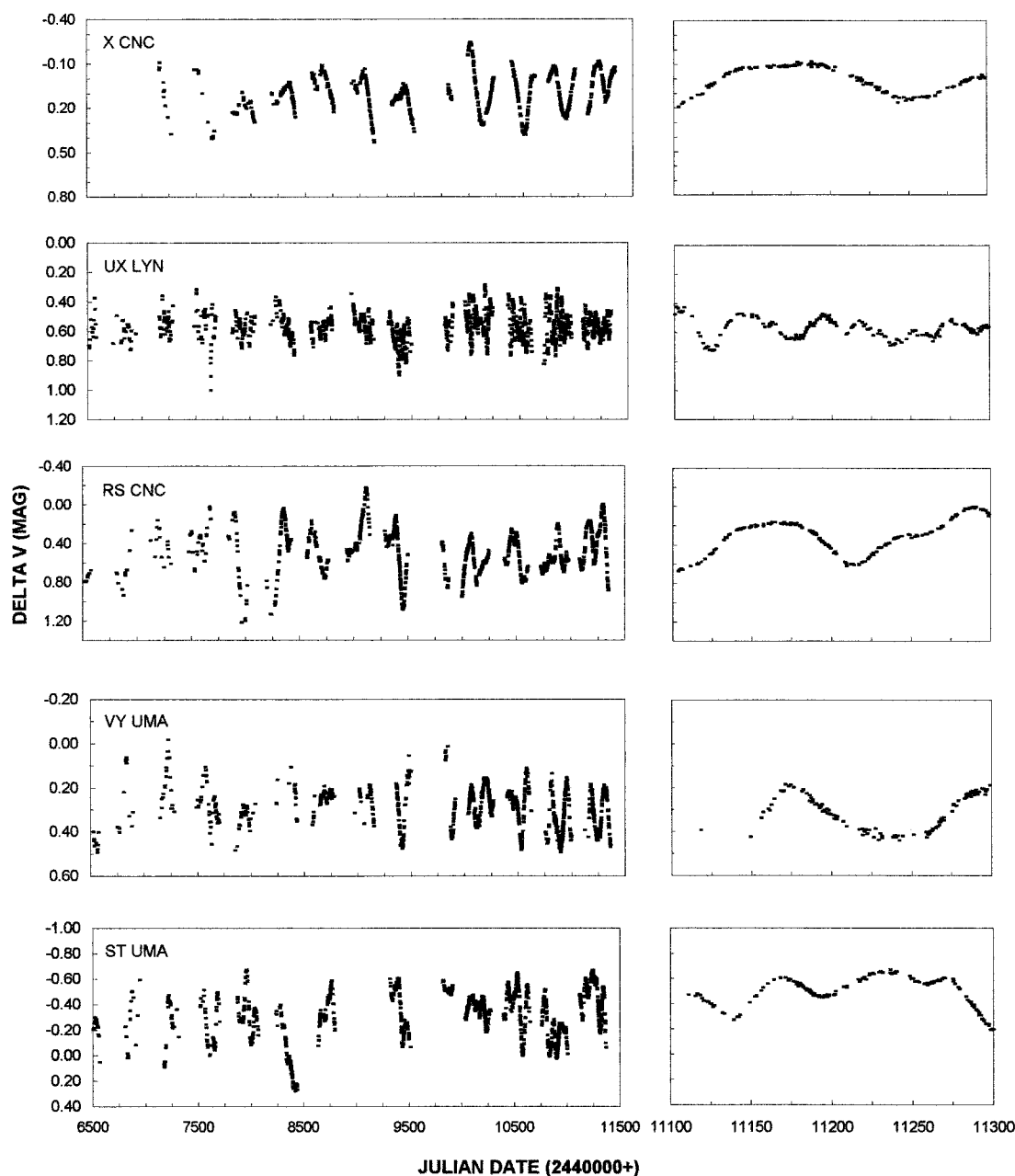
FIG. 4.—Differential V light curves of X Cnc, UX Lyn, RS Cnc, VY Uma, and ST Uma, relative to the comparison stars listed in Table 1.
