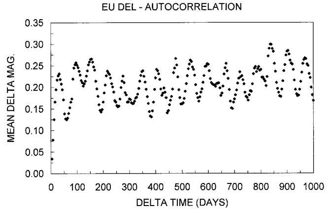
FIG. 14.—Autocorrelation diagram for EU Del, showing minima at multiples of 63 days, indicating a strict underlying periodicity in this star.
