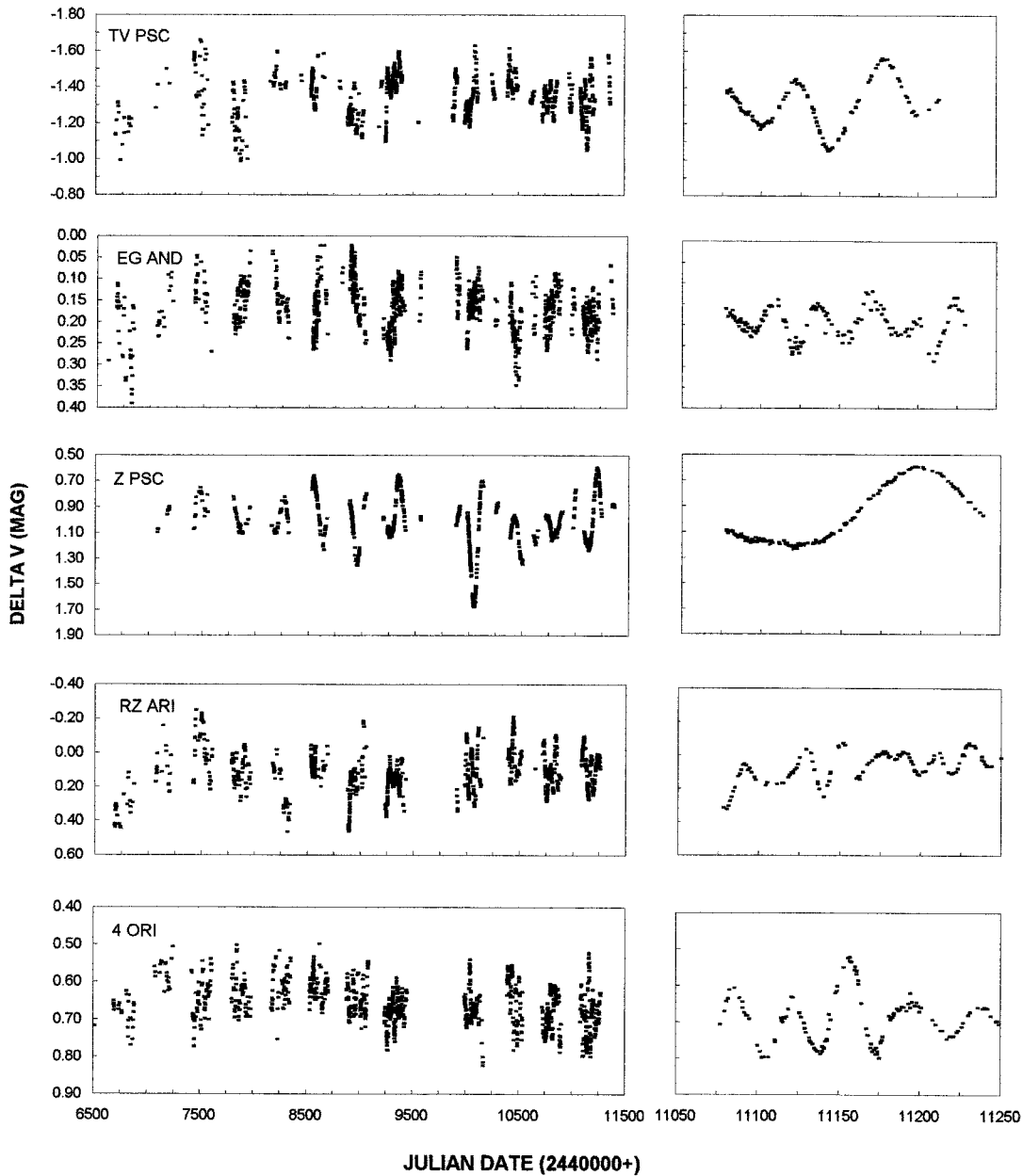
FIG. 1.—Differential V light curves of TV Psc, EG And, Z Psc, RZ Ari, and 4 Ori, relative to the comparison stars listed in Table 1.
