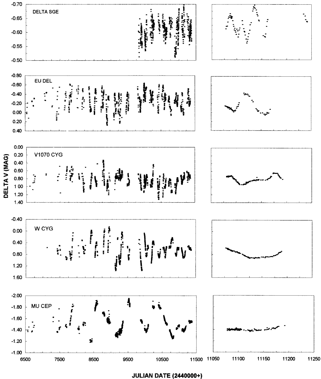
FIG. 7.—Differential V light curves of \delta Sge, EU Del, V1070 Cyg, W Cyg, and \mu Cep, relative to the comparison stars listed in Table 1.
