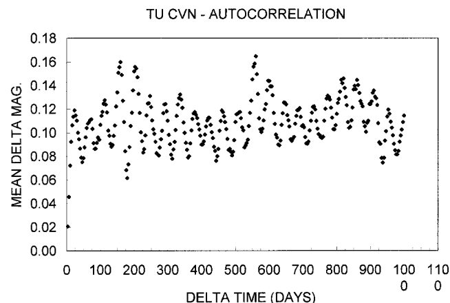
FIG. 11.—Autocorrelation diagram for TU CVn, showing 22 minima in 980 days, or a strict period of 44.5 days.
