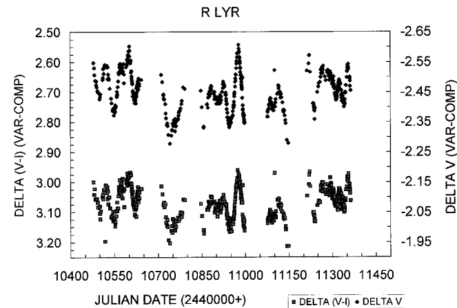
FIG. 13.—Light and color curves for R Lyr, showing the correspondence between the V–I color curve and the V light curve, and also showing the complex variations.
