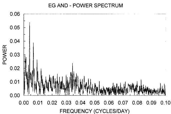
FIG. 9.—Power spectrum for EG And, showing peaks corresponding to periods of 29 and 242 days. This star shows conspicuous variations on both timescales.
