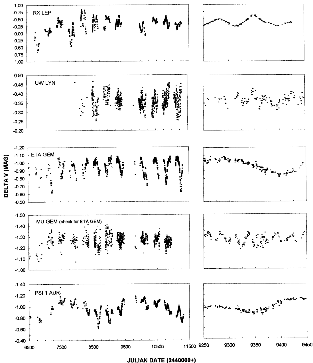
FIG. 2.—Differential V light curves of RX Lep, UW Lyn, \eta Gem, \mu Gem (check star for \eta Gem), and \psi^1 Aur, relative to the comparison stars listed in Table 1.
