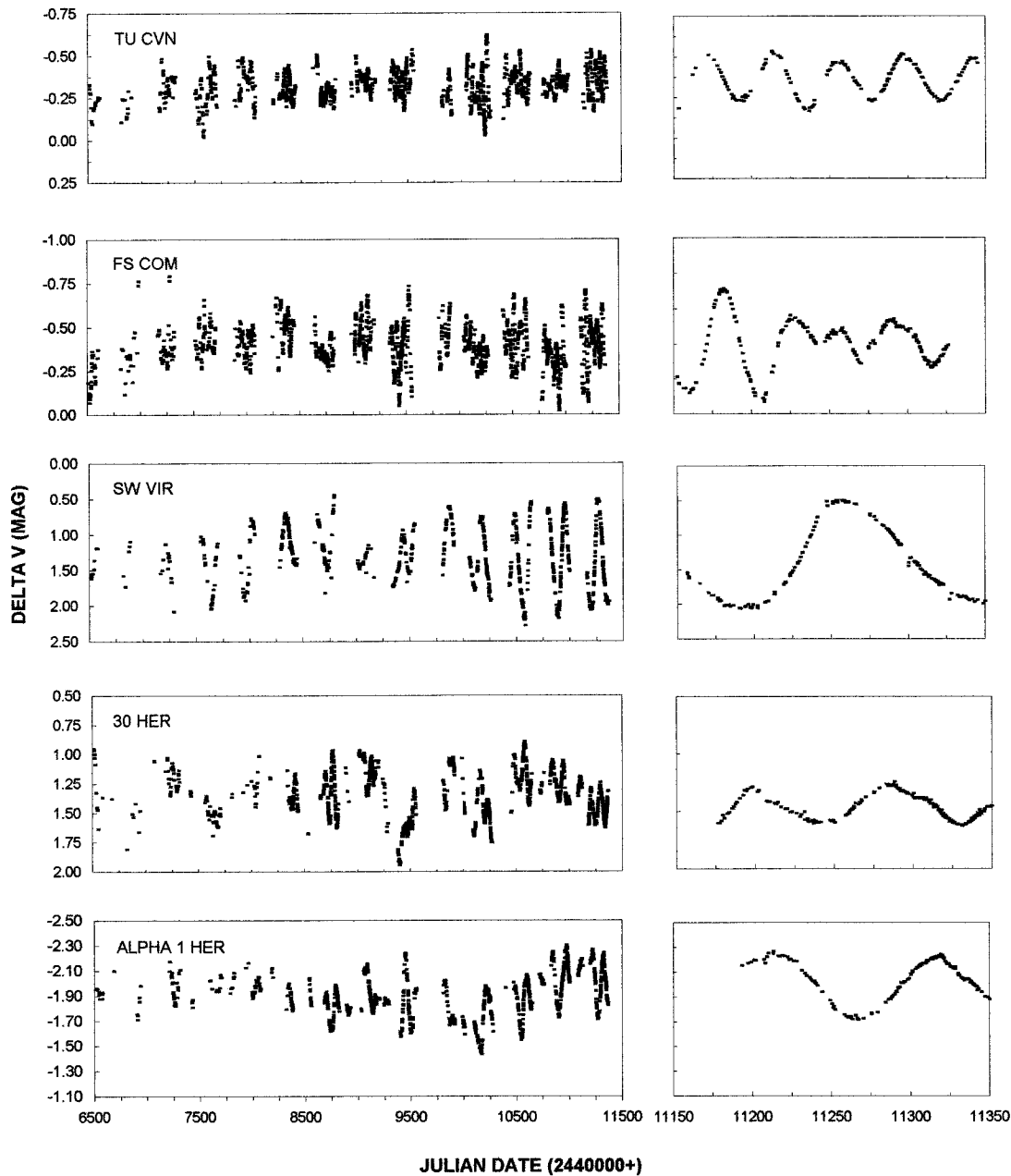
FIG. 5.—Differential V light curves of TU CVn, FS Com, SW Vir, 30 Her, and \alpha^1 Her, relative to the comparison stars listed in Table 1.
