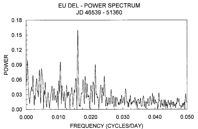
FIG. 15.—Power spectrum for EU Del, showing a conspicuous peak corresponding to a period of 63 days. The alias structure is complex; the two secondary peaks are separated by 2 cycles yr -1 from the main peak.
