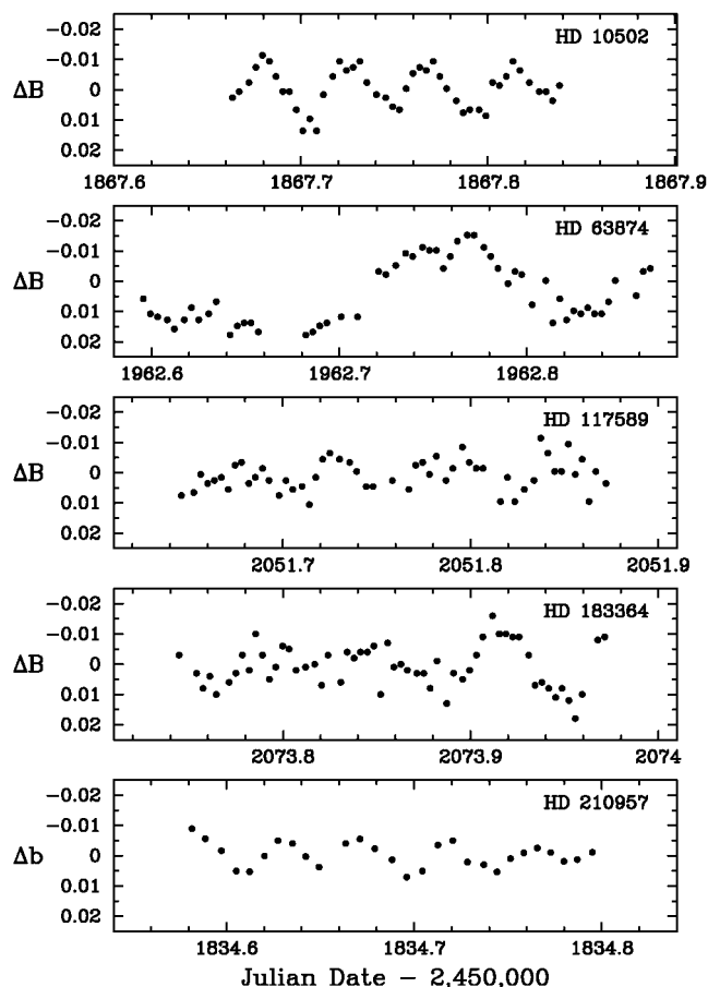
FIG. 1.—Differential Johnson B or Strömgren b photometric observations of each of the new \delta Scuti stars acquired over several hours on a single night near each star's time of opposition. The differential magnitudes are computed relative to the mean brightness level for the night. All five panels are plotted to the same scale and show high-frequency, low-amplitude photometric variations typical of \delta Scuti variables.
