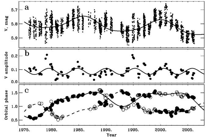
FIG. 1.—Activity patterns on HR 1099. (a) All V -magnitude observations analyzed in this Letter. The data before 1993 are from Henry et al. (1995). Cyclic variations of the mean brightness are revealed with a harmonic fit (solid curve) with a period of \sim 15 years. (b) Peak-to-peak amplitude of the light curves (filled circles). A harmonic fit (solid curve) reveals the period of 5.3 \pm 0.1 yr. (c) Phases of the spots recovered with the light-curve inversions. Filled circles denote the larger or single active region observed at a given time, while open circles indicate a second, smaller region if observed. Migration paths of the ALs are indicated with solid and dashed curves, which are harmonic fits to the measurements with a long-term trend. The migration pattern is apparently repeated in about 16 years.
