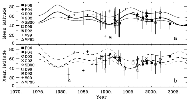
FIG. 3.—Butterfly diagram of HR 1099. (a) Mean latitudes recovered from the fit to the active longitude shown in Fig. 1c as the solid curve. (b) Mean latitudes recovered from the fit to the active longitude shown in Fig. 1c as the dashed curve. In both plots, the mean latitudes of spots in the opposite hemispheres measured from DI are shown with different symbols corresponding to the following sources: VP83 (Vogt & Penrod 1983), V99 (Vogt et al. 1999), D92 (Donati et al. 1992), D99 (Donati 1999), SB00 (Strassmeier & Bartus 2000), G03 (García-Alvarez et al. 2003), D03 (Donati et al. 2003), P04 (Petit et al. 2004), and P06 (P. Petit 2006, private communication). Standard deviations of the mean DI latitudes (if several spots were observed) are shown as vertical dashes. The thick curves are the solutions using the best parameters of the differential rotation law by Petit et al. (2004). The thin curves indicate the \pm 1 \sigma interval for the best parameters obtained in this Letter (filled circle in Fig. 4). The two solutions are statistically equivalent.
