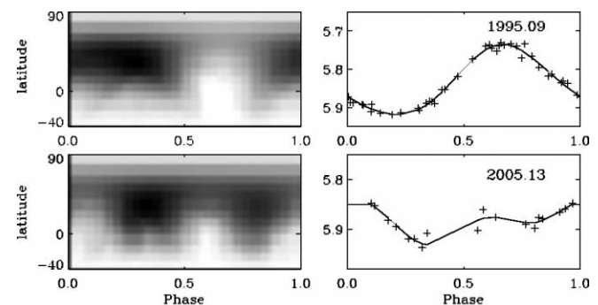
FIG. 2.—Examples of the spot filling factor distribution on HR 1099 (left) and corresponding light curves (right). The stellar surface was modeled with a grid of 10^\circ \times 10^\circ . The spot filling factor at each grid point indicates relative contributions from two temperature components, the hot photosphere and cool spots. In the images, the darker area implies a higher spot filling factor. Observed light curves are shown as crosses, and the fit as the solid line. In contrast to direct modeling of light curves, the inversions do not involve any assumptions about spot shapes, numbers, or latitudes.
