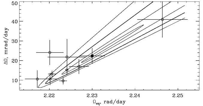
FIG. 4.—The \chi^2 surface contours for the two parameters in eq. (2) calculated from the AL migration and the DI mean spot latitudes. The \chi^2 = 1 level is emphasized by a thick contour. The best-fit solution is indicated by the filled circle. The measurements by Petit et al. (2004) are shown as open circles. The strongly elongated shape of the minimum implies that the two parameters are almost linearly dependent. The distribution of the measurements along the major axis of the error ellipsoid suggests that they reflect errors in DI spot latitudes rather than true variations of the differential rotation.
