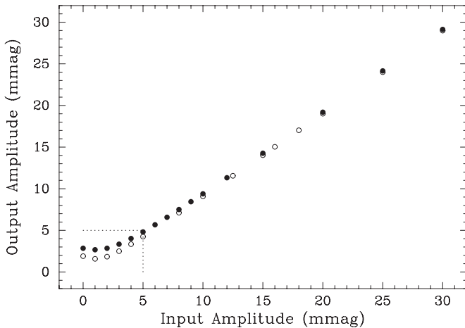
Figure 9. Relation between artificial input signals at the orbital frequency in our noisy light curves and their recoveries by periodogram analysis. The recovery is linear and hence reliable to a level of \approx 5 mmag (faint dotted lines).
