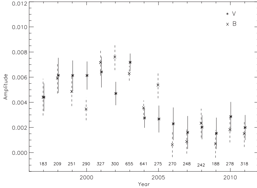
Figure 6. Full amplitudes of the rotational signature in B and V for each of the 15 observing seasons. These values were determined by rectifying the seasonal means to a common value and then prewhitening the 15 year B and V data sets for several periods consistent with the long cycles found in various individual seasons. The numbers of V observations in each season are given at the bottom of this and the following figure.
