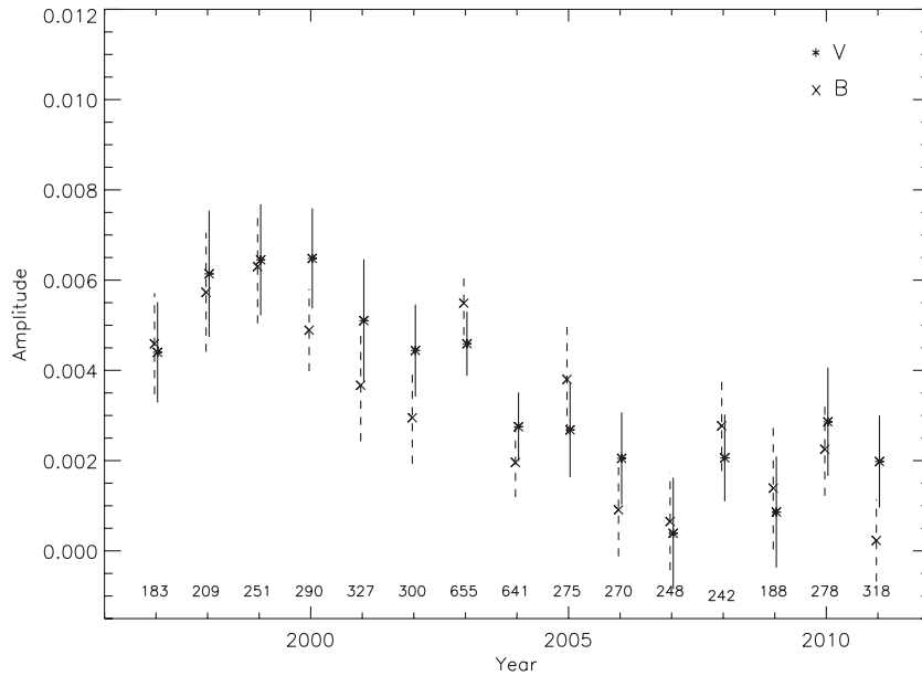
Figure 7. Full amplitudes of the rotational signature in B and V for the 15 individual seasons in our study. These values were determined from the light-curve residuals after removing the long-cycle modulations found in SHV and in Figure 4.
