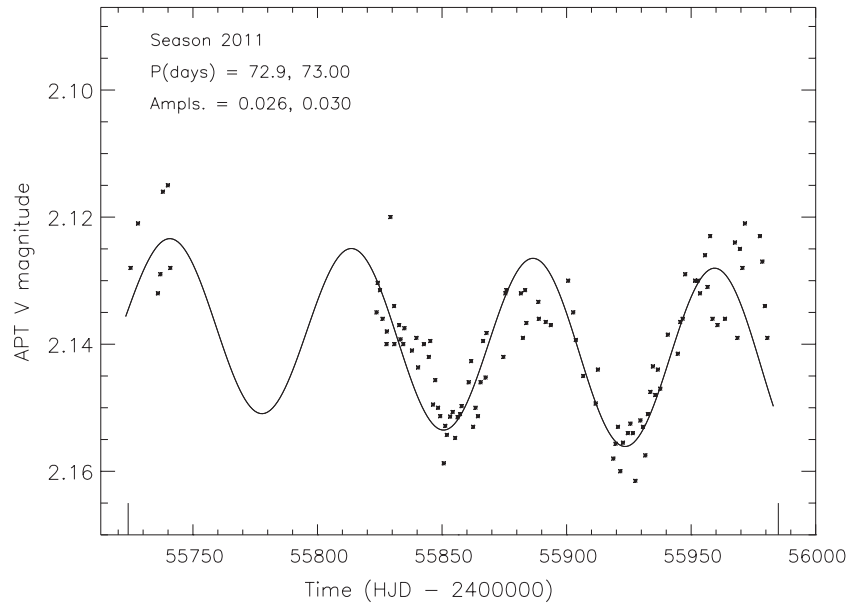
Figure 5. V-band photometry of \gamma Cas showing the long cycles of season 2011. Note the trend to fainter magnitudes after reaching a maximum in mid-2011 following the 2010 “outburst.”
