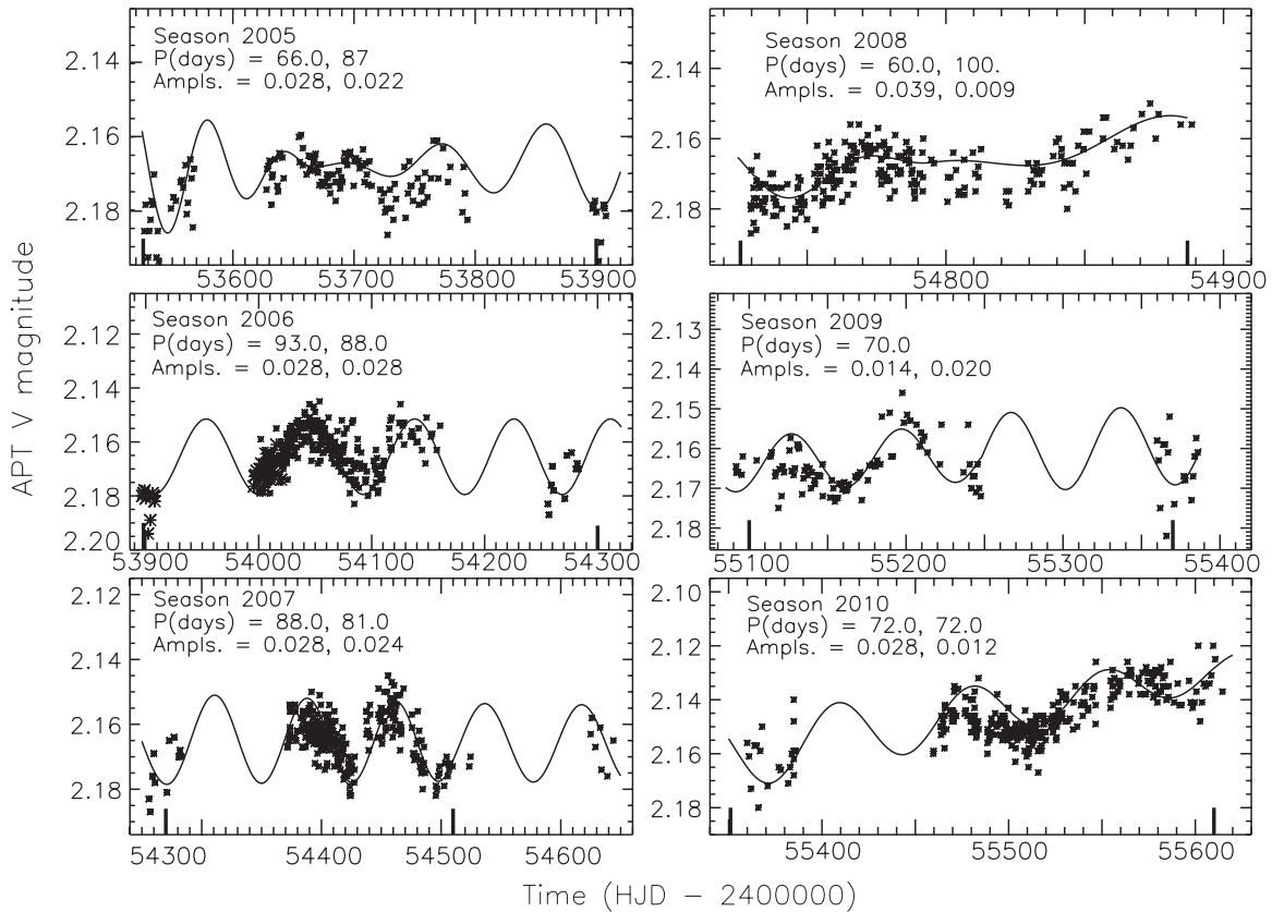
Figure 4. V-band photometry of \gamma Cas showing the light curve during seasons 2005–2010, ending in 2011 February. The approximate date of the immediate post-maximum of 2010–2011 is indicated by a small clump of points at 2011.5. The solid line indicates the damped or changing sinusoids needed to fit the data. Their combs at the bottom of the panels show the reference start and end times for the computation of these sinusoids using the periods and amplitudes indicated.
