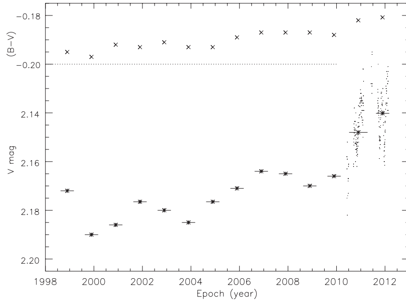
Figure 1. Johnson V ( m_V ) magnitudes (asterisks) and (B - V) color indices (crosses) of \gamma Cas acquired with the T3 APT at Fairborn Observatory during the 1998–2011 observing seasons; large symbols represent seasonal means. Error bars on the means are smaller than the symbol size. Horizontal bars denote the coverage for a seasonal mean time. Small dots indicate individual m_V measurements in the 2010 and 2011 seasons. All magnitudes in this paper are plotted with brightness increasing upward.
