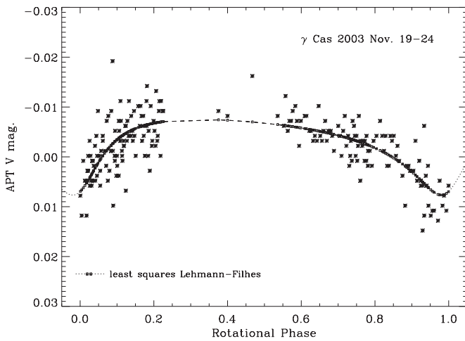
Figure 8. Light curve of the V residuals for 2003 November 19–24 (RJD 52,962–52,967) phased to a period of 1.21581 days. Symbols refer to observations taken on different nights during this interval. The solid line is the fit from a least-squares Lehmann–Filhes solution ( e = 0.49 , \omega = 40^\circ ).
