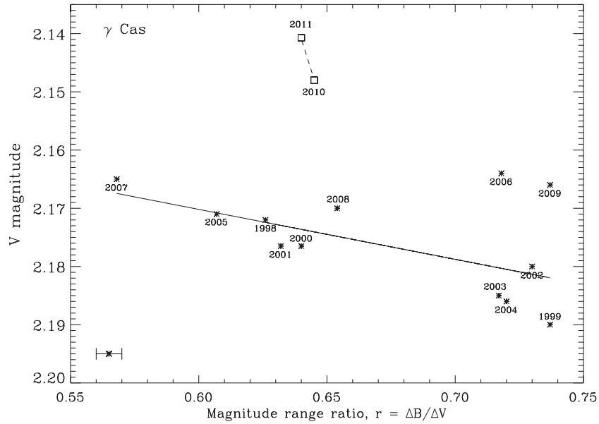
Figure 2. Seasonal quantities r = \Delta B/\Delta V discussed in the text plotted against seasonal V means for \gamma Cas. For each of the two filters, the “ \Delta ” quantity is the mean of the absolute values of all observations in a season with respect to the seasonal average. Season annotations are indicated near each plotted point. The solid line is the regression fit through the points, except for the 2010 outburst and 2011 decline intervals.
