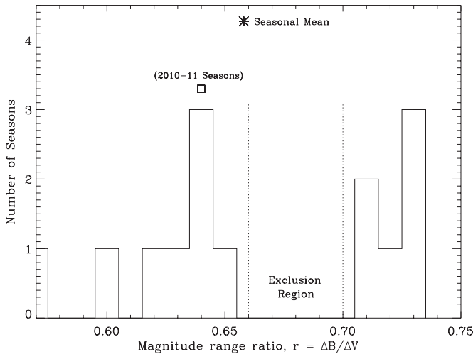
Figure 3. Histogram of the r values (defined as in Figure 2). To a modest level of significance the distribution is bimodal. The mean r for all seasons, except the anomalous seasons 2010 and 2011, is shown by an asterisk. The mean value of the last two seasons is labeled separately.
