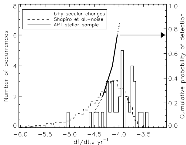
Fig. 2. A histogram of stellar secular behavior as measured by the fractional rate of change of b + y photometric flux with time, (\frac{df}{dr})_{15} , for a sample of 34 stars observed with Automated Photoelectric Telescopes. The subscript “15” means that \frac{df}{dr} was derived from a time series of 15 years duration. Also shown are commensurate histograms from the time series of the reconstruction of Shapiro and colleagues, computed as described in the text. The sloped line near x = -4.2 shows the probability that the given value of (\frac{df}{dr})_{15} will be detected in the stellar sample, evaluated using the statistical properties of the photometric standard stars used.
