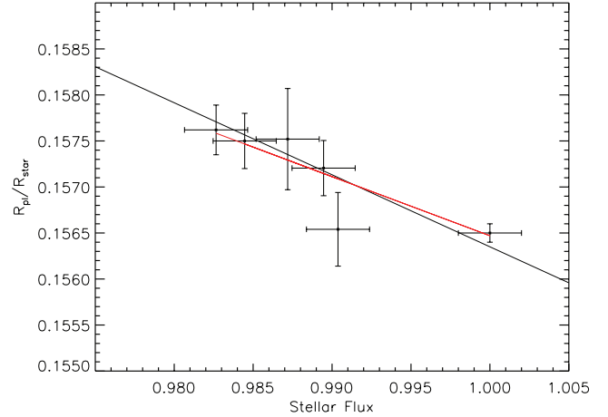
Figure 12. HST planet-to-star radius measurements ( R_{\text{pl}}/R_{\text{star}} ) between 5200 and 6100 \text{ \AA} from STIS G430L, STIS G750M and ACS HRC plotted against the observed stellar flux at the transit epoch. The black solid line is the predicted relation for the radius impact from stellar variability, assuming non-occulted dark stellar spots. The red line is the best-fitting relation from the HST observations, which is in very good agreement with the prediction.
