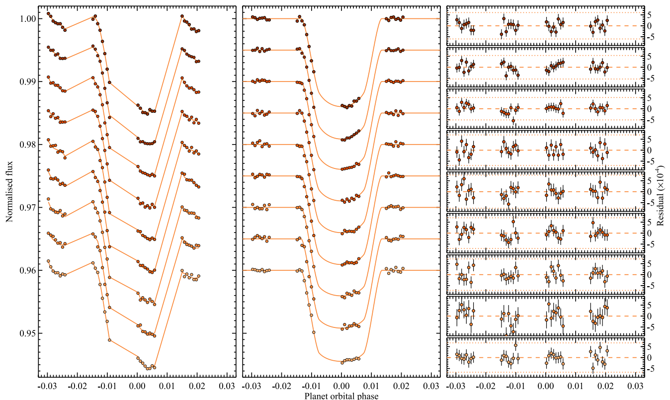
Figure 10. Same as Fig. 8, but for the HST /STIS G750L data, obtained on UT 2012 May 30 (visit 20).
